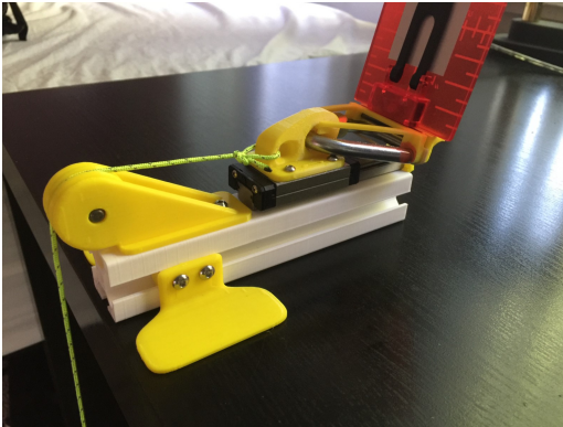
1. Clamp Line Rig at Edge of Flat Surface. Attach required weights to leader line.
