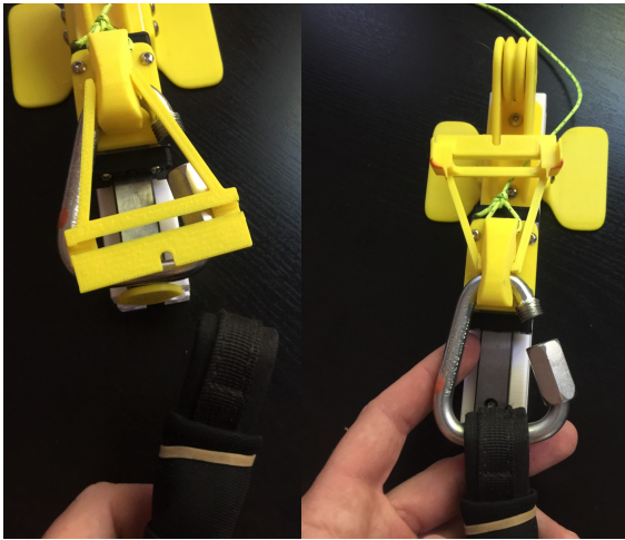
4. Place Rubber Band Around Riser and Attach to Maillon, Close.
