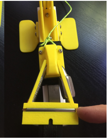
5. Secure Laser Target Mount with Rubber Band. Replace Steel Rod for Laser Target Mounting.
