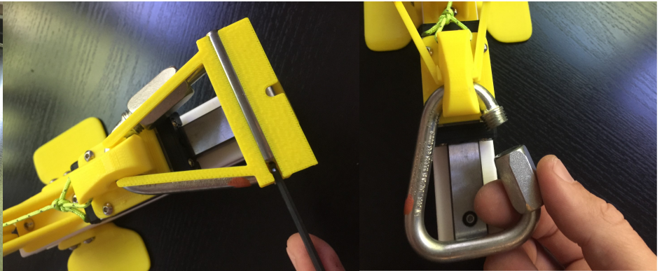
2. Push out Steel Rod with Allen Wrench or Screwdriver.
