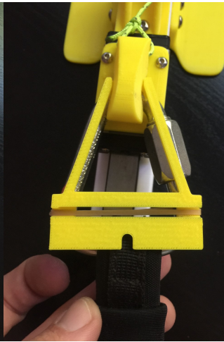
5. Secure Laser Target Mount with Rubber Band. Replace Steel Rod for Laser Target Mounting.
